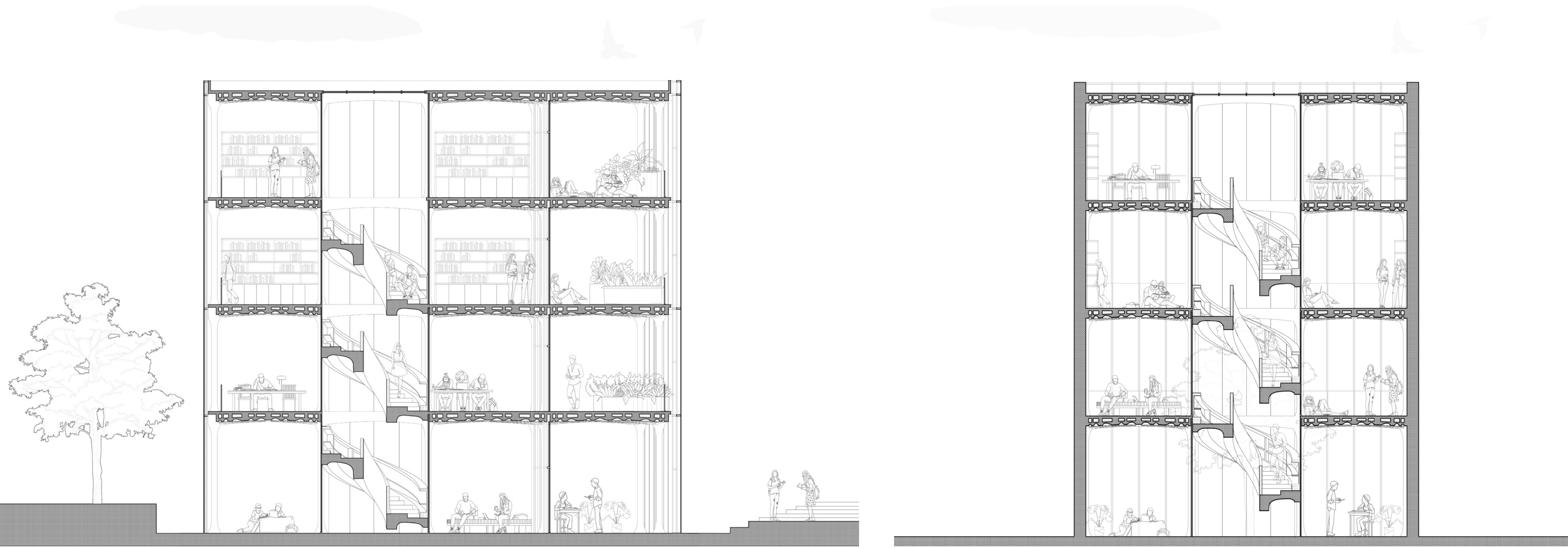
Section A-A Section B-B
