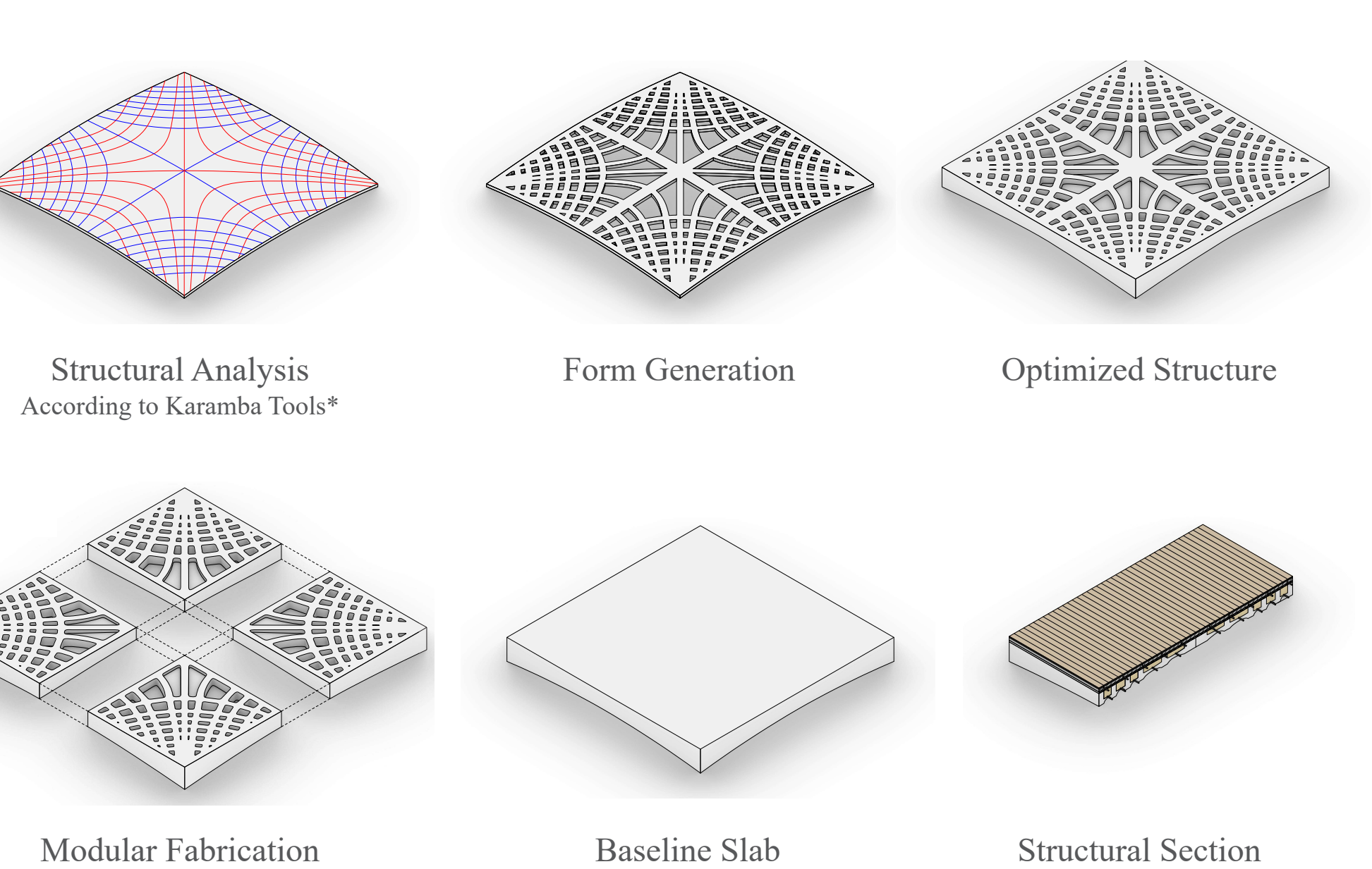
Development of the Slabs
