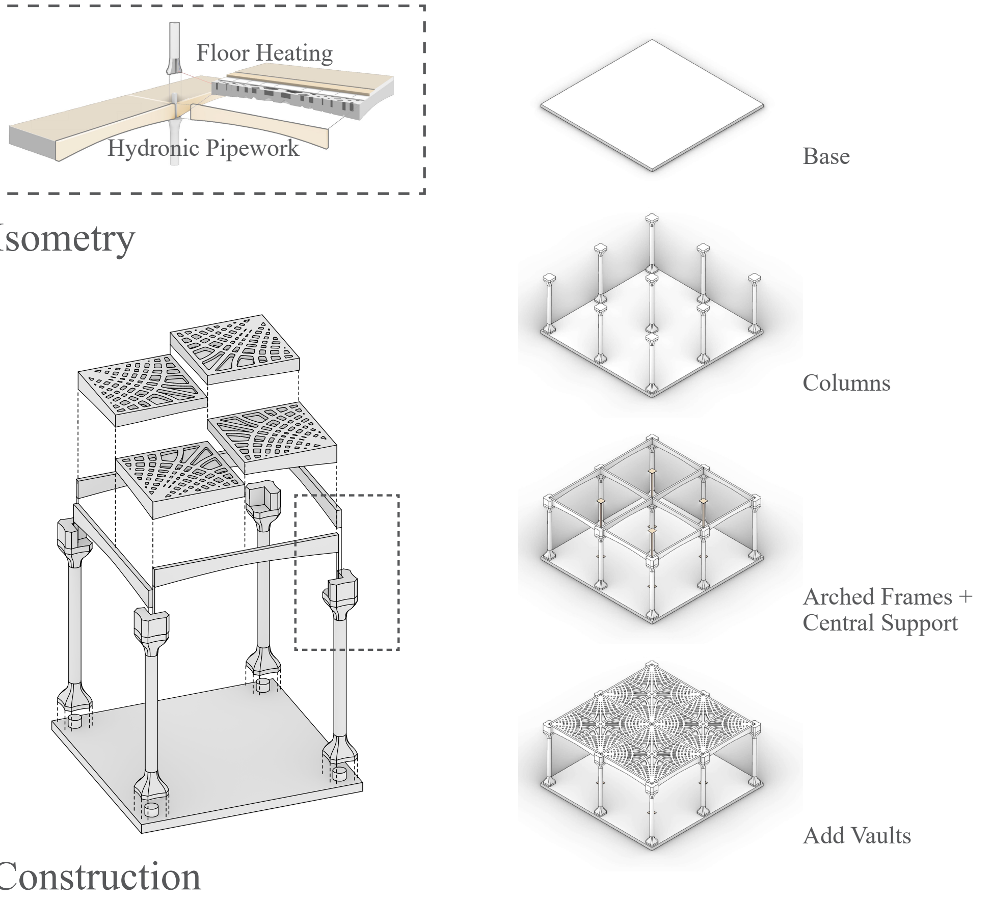
Development of the Slabs
