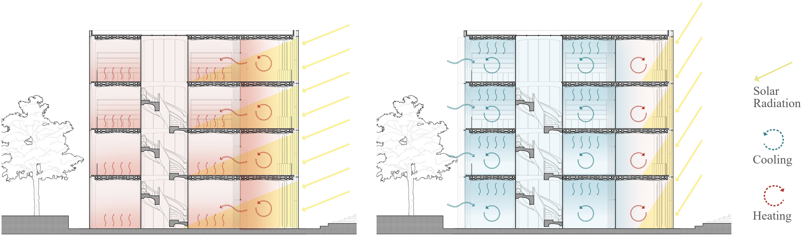
Climate Concept Winter: 17° (Min. Incidence angle) Summer: 64° (Max. Incidence angle)
